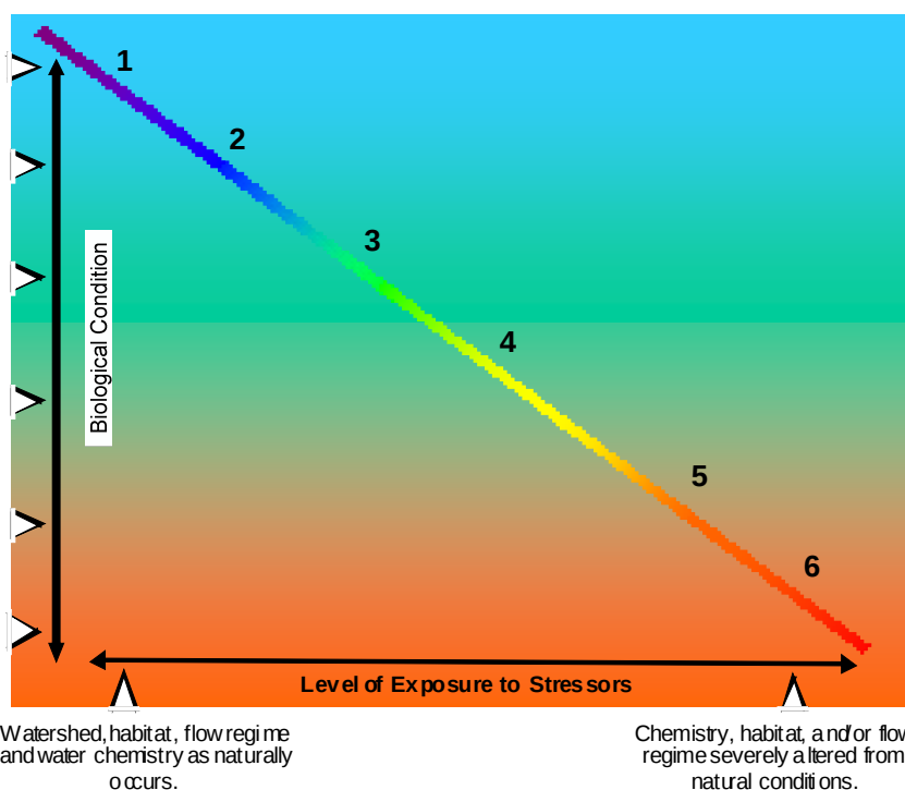
Figure 7. The Biological Condition Gradient (BCG) conceptual model that depicts six levels of change in key biological attributes in response to the increasing effect of stressors (modified from Davies and Jackson (2006).
